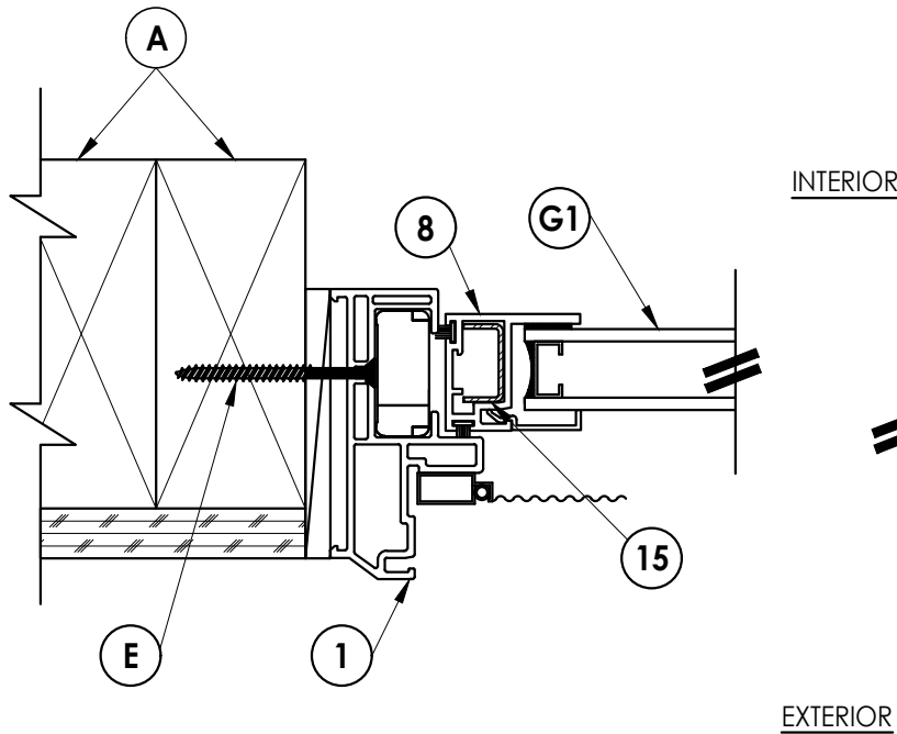
1 5 HORIZONTAL CROSS SECTION Wood stud construction
