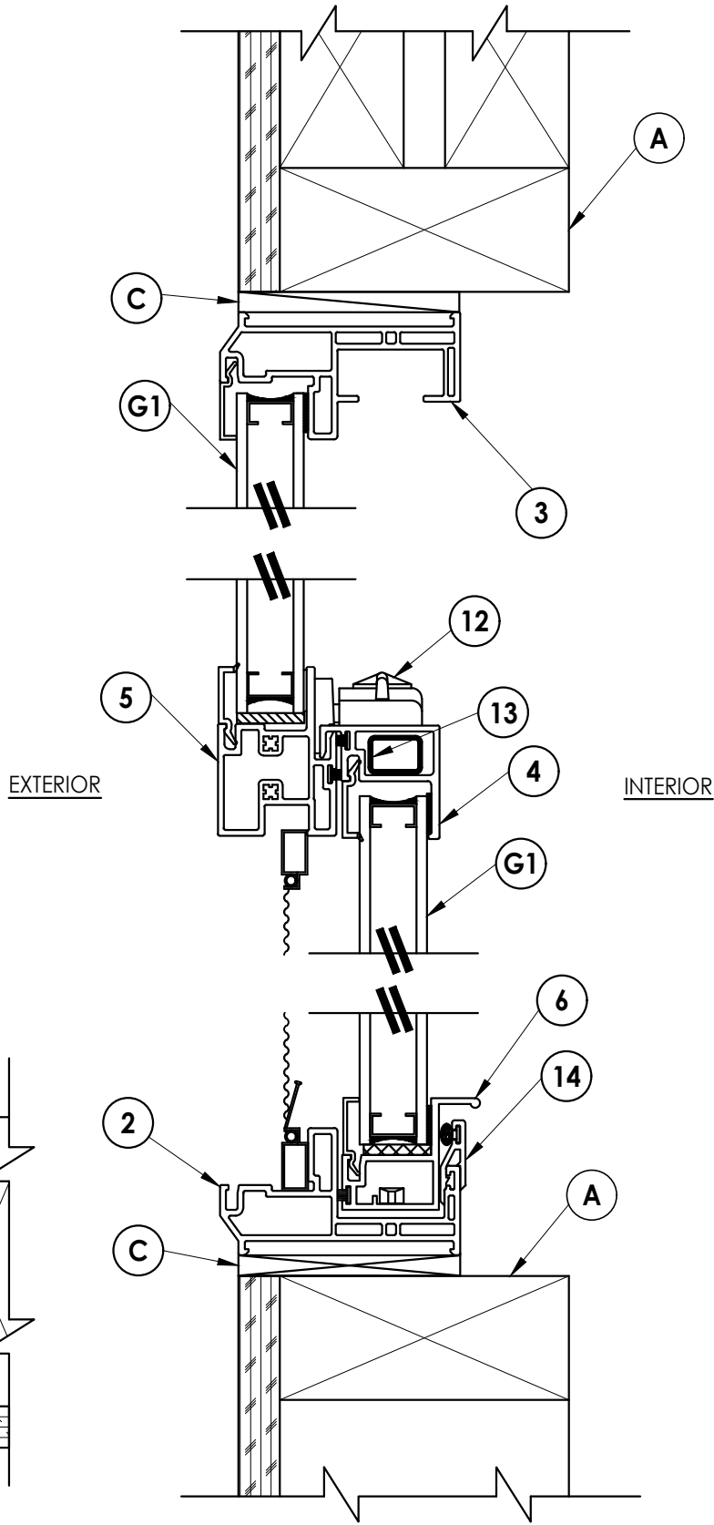
3 5 VERTICAL CROSS SECTION Wood stud construction
