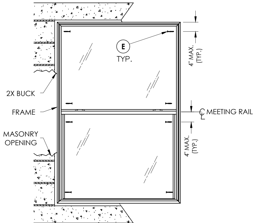
2X FRAME ANCHORING Masonry Construction
